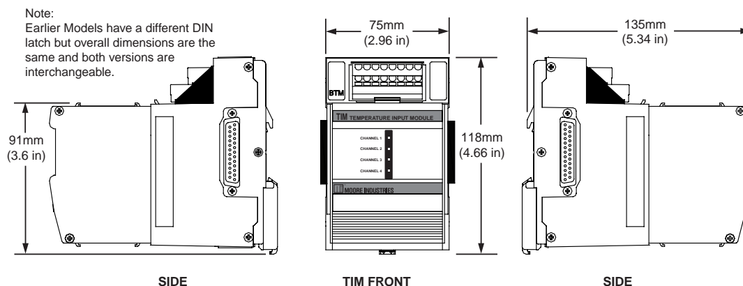
Figure 17. TIM Dimensions
