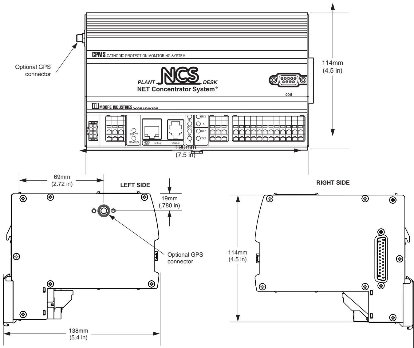
Figure 1. CPMS Dimensions
