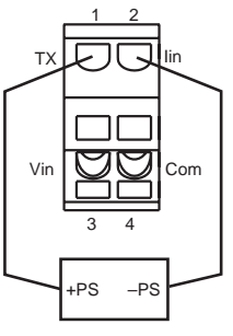
Current input with Transmitter Excitation
