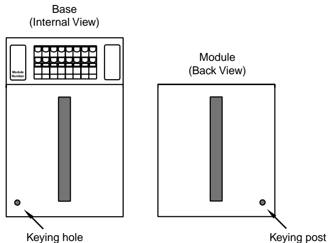
Figure 10. Snapping in a New Module
