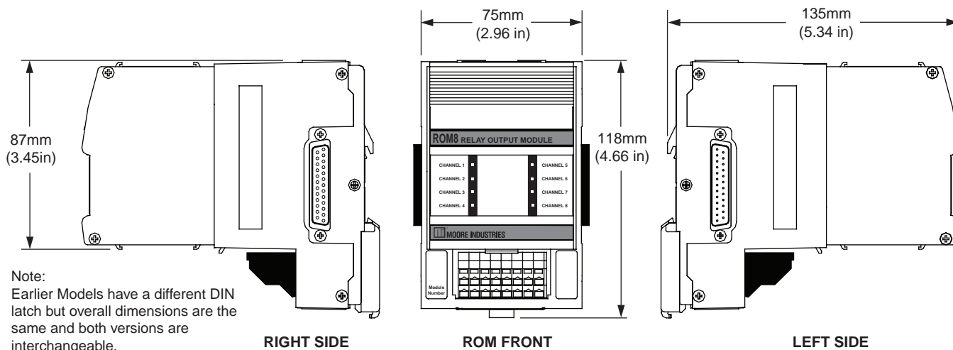
Figure 28. ROM Dimensions
