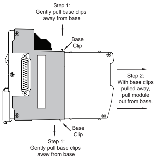
Figure 9. Removing the Old Module
