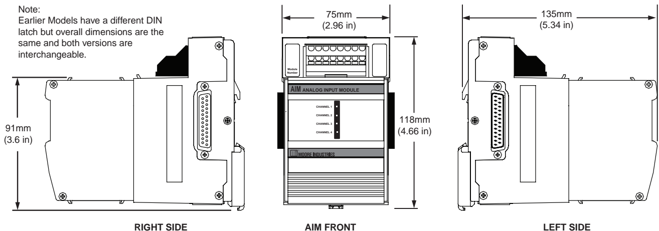
Figure 14. AIM Dimensions
