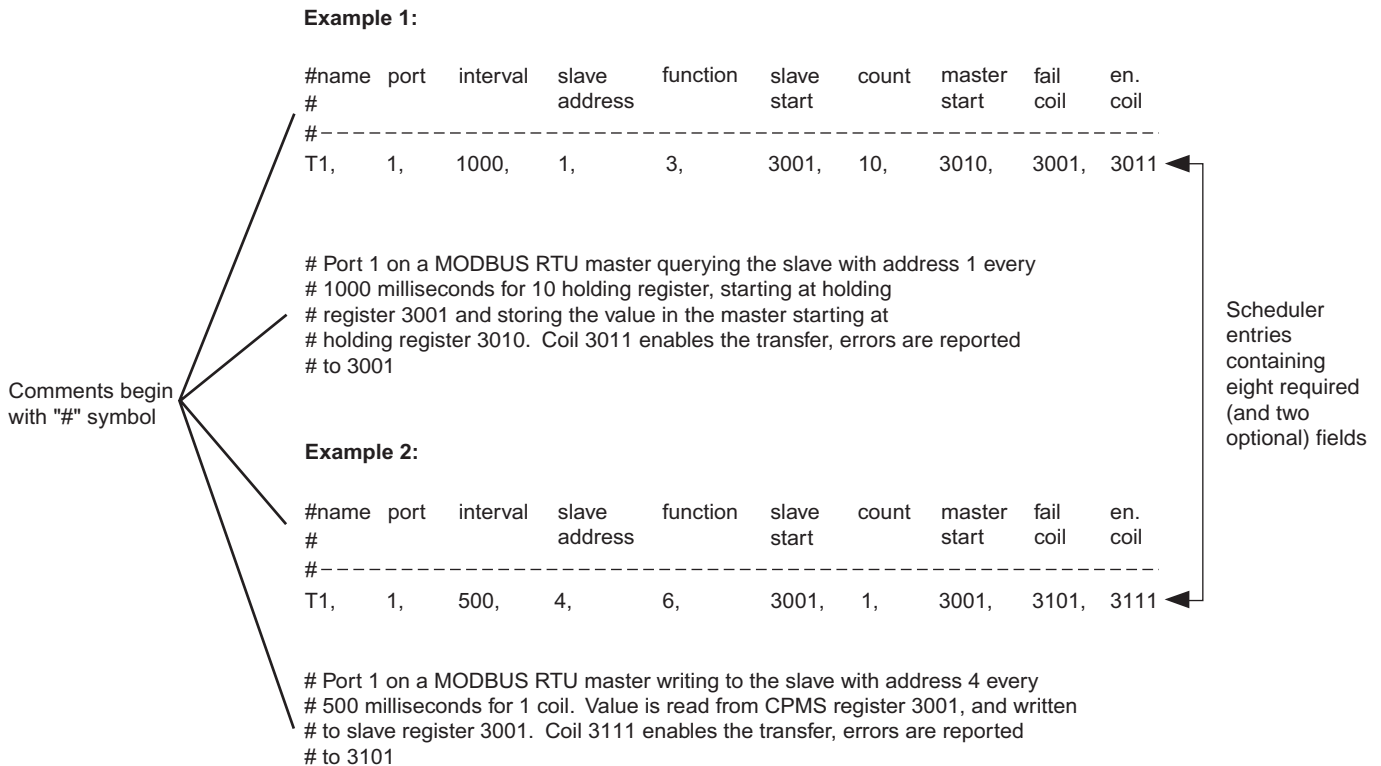
Figure 6. Example of Scheduler Entries
