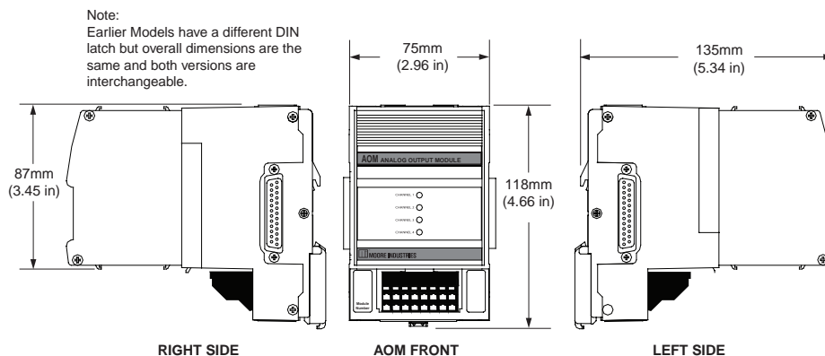
Figure 20. AOM Dimensions
