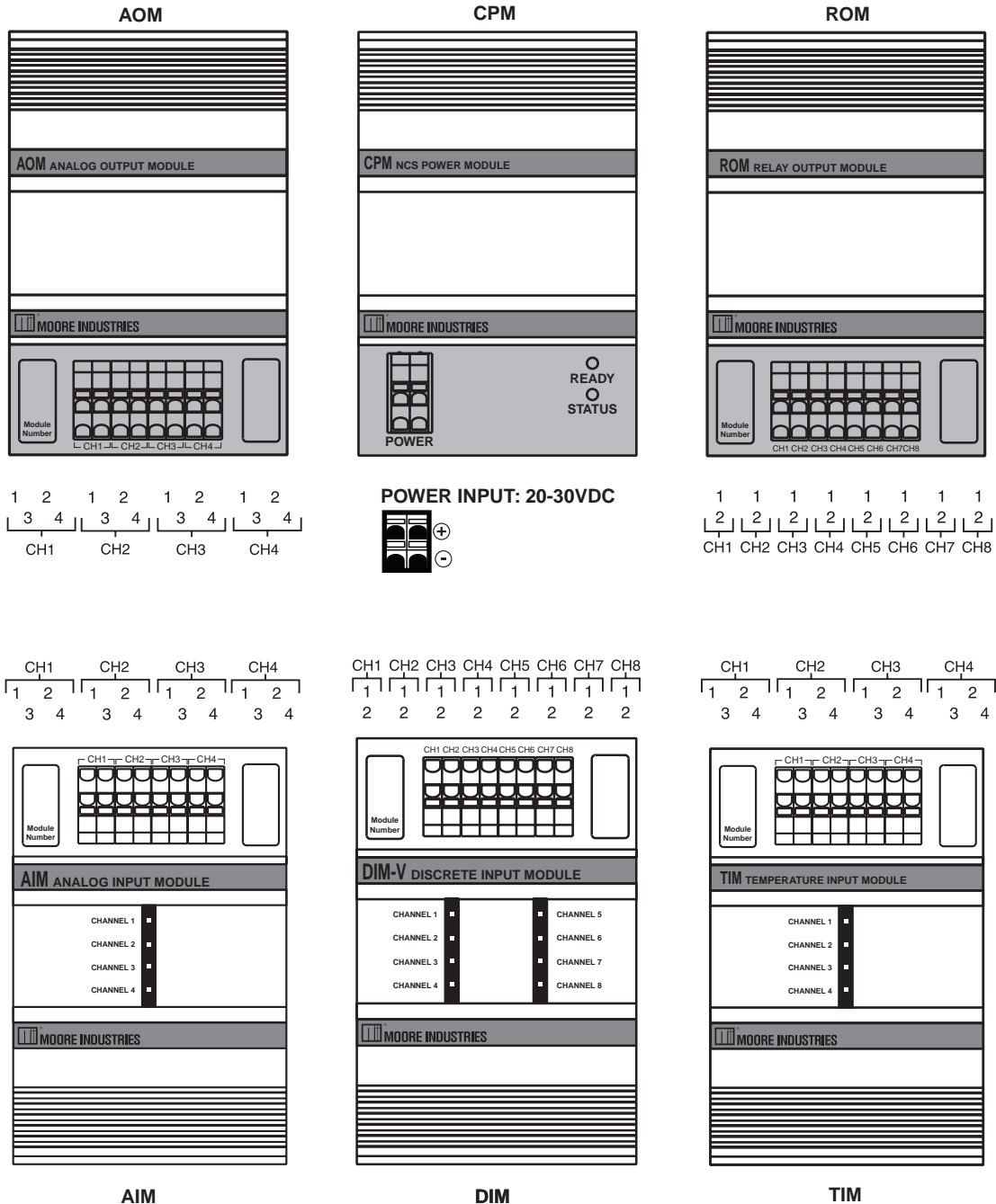
Figure 31. Terminal Designations of CPMS I/O Modules
