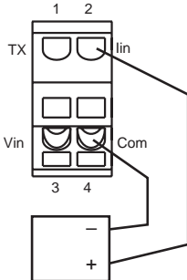
Current input without Transmitter Excitation
