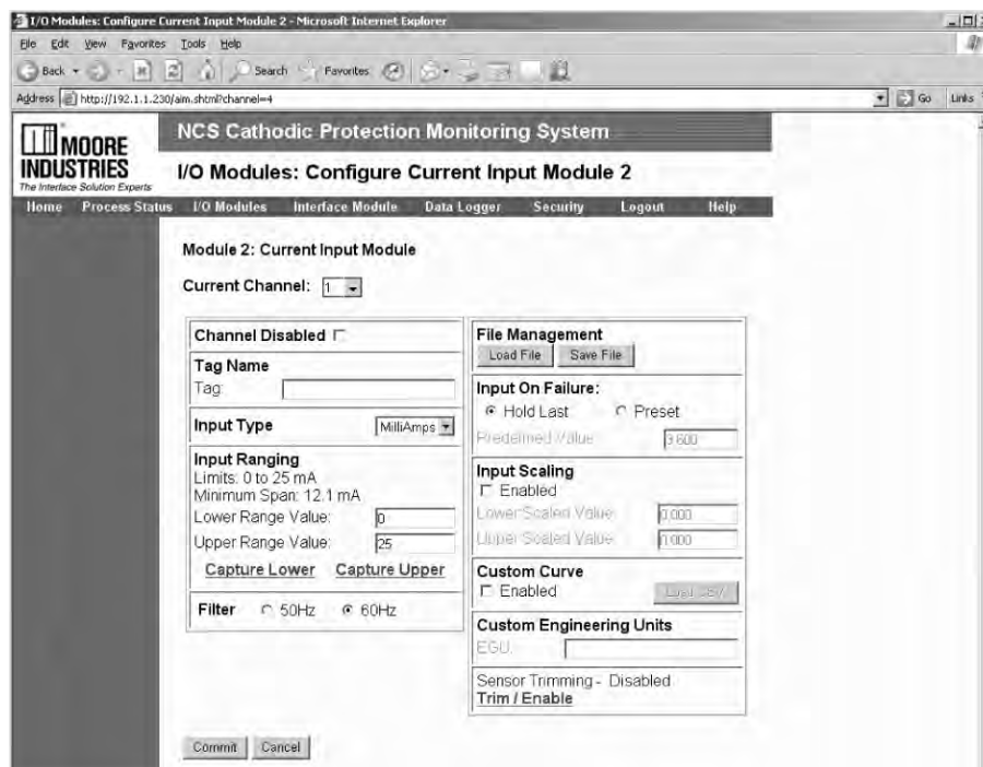
Figure 12. Current Channel Configuration Web Page
