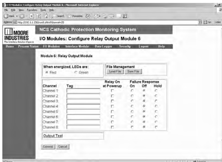
Figure 30. ROM Configuration Web Page
