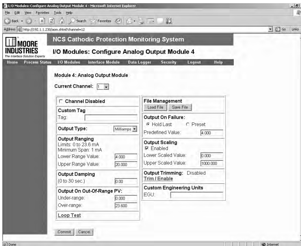
Figure 19. TIM Configuration Web Page
