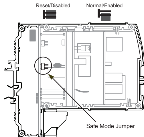
Figure 8. Safe Mode Jumper Location
