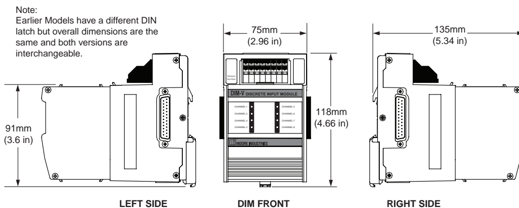
Figure 25. DIM Dimensions
