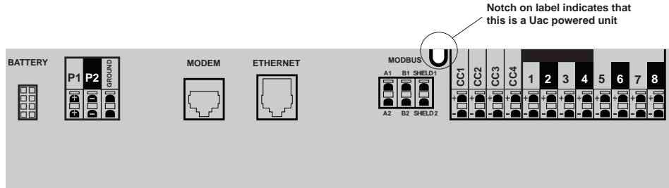
Figure 2. CPMS Terminal Layout
