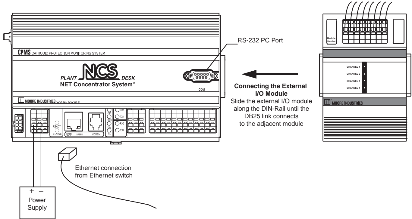
Figure 3. CPMS Connection Diagram
