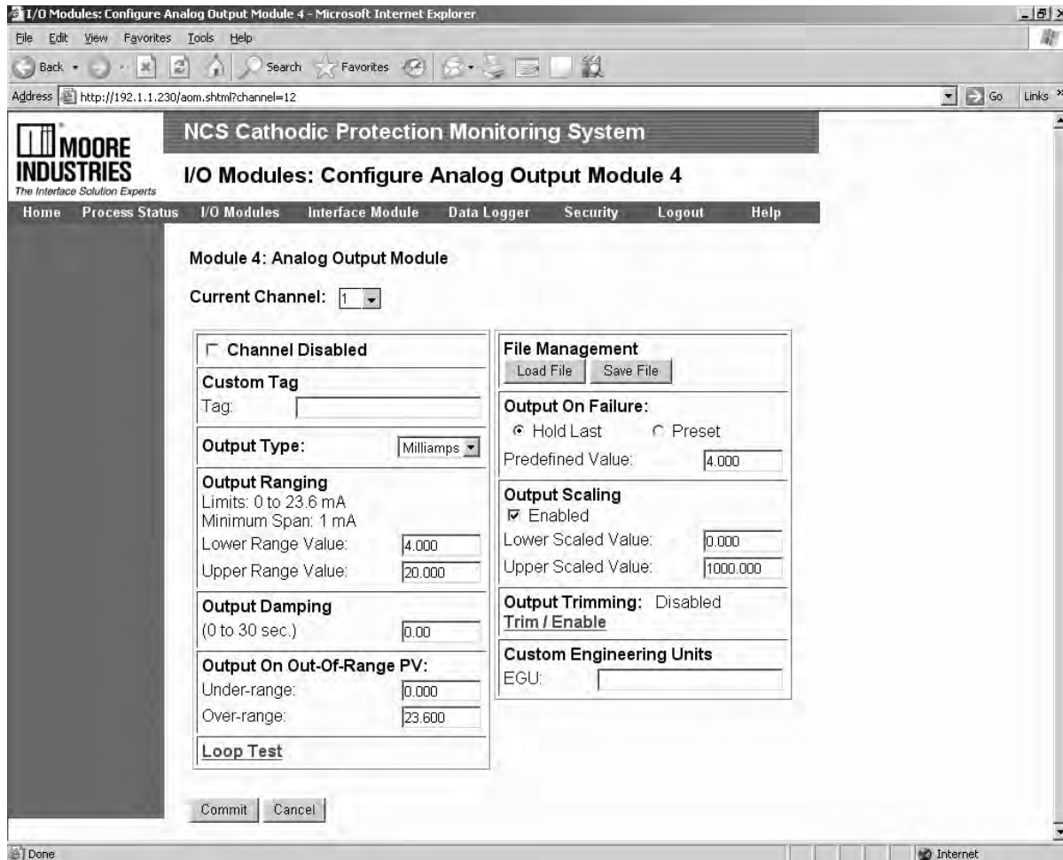
Figure 22. AOM Configuration Web Page
