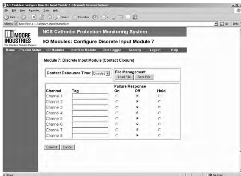
Figure 27. DIM Configuration Web Page
